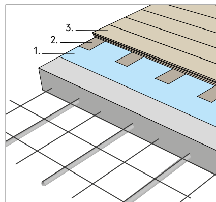
Laying solid wood flooring.
