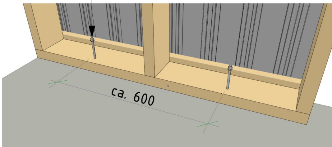
M8 Expander
